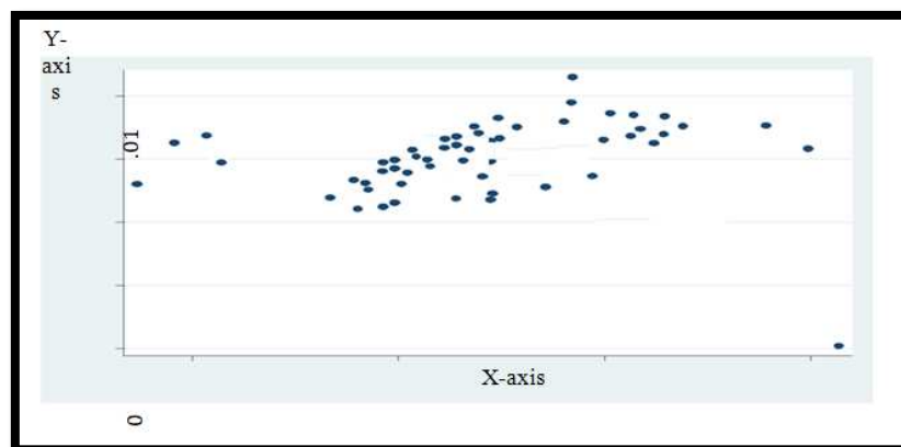
Figure 1: Heteroscedasticity
